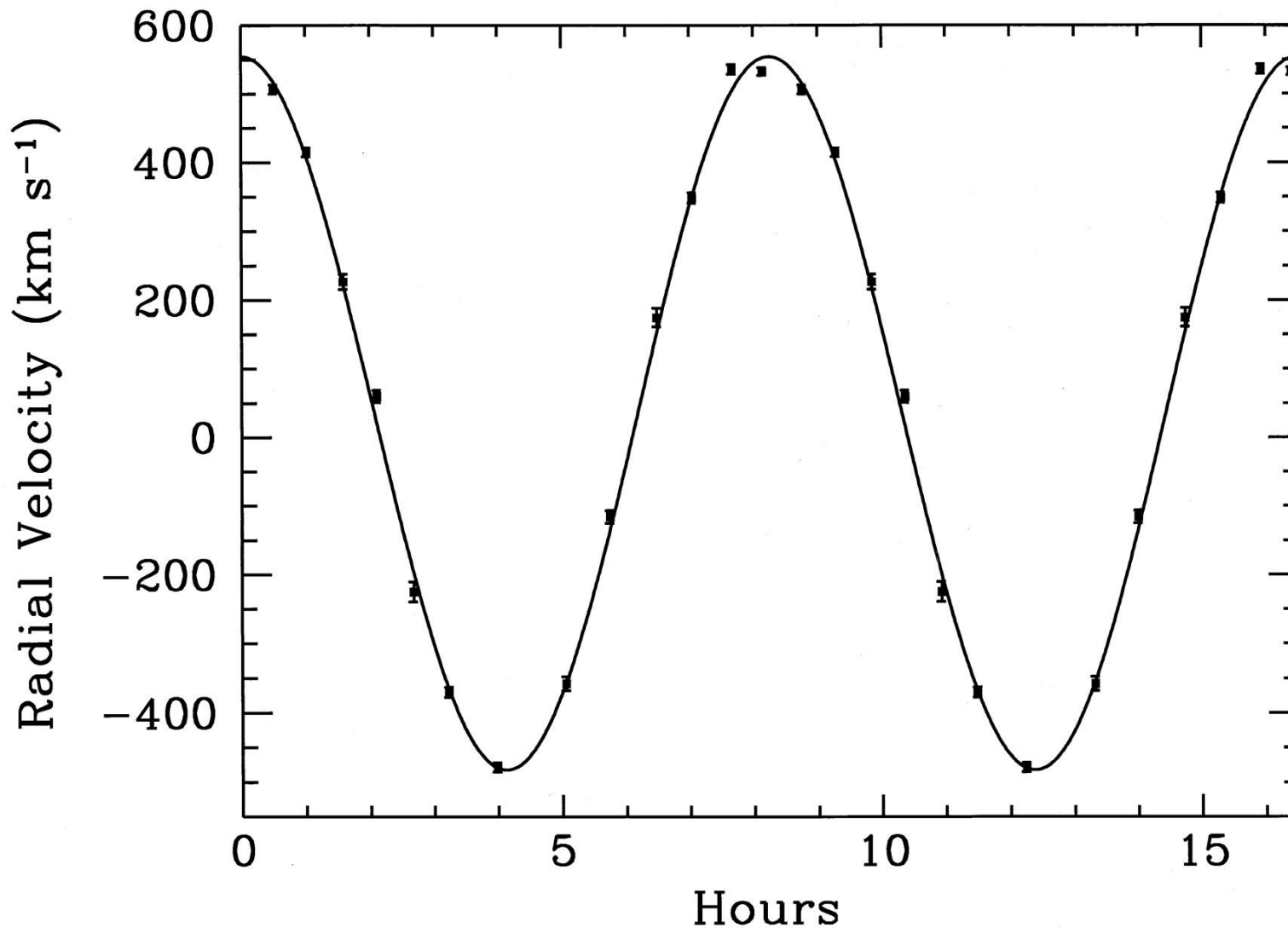
Radial-velocity curve of the visible star in the X-ray binary GS 2000 + 25. (From Filippenko et al. (1999) www.pnas.org/content/96/18/9993.full ) Shows that invisible, compact, companion star is a 5 solar mass black hole.
