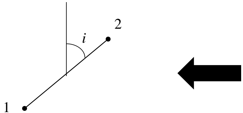
Inclination of orbit to line of sight
