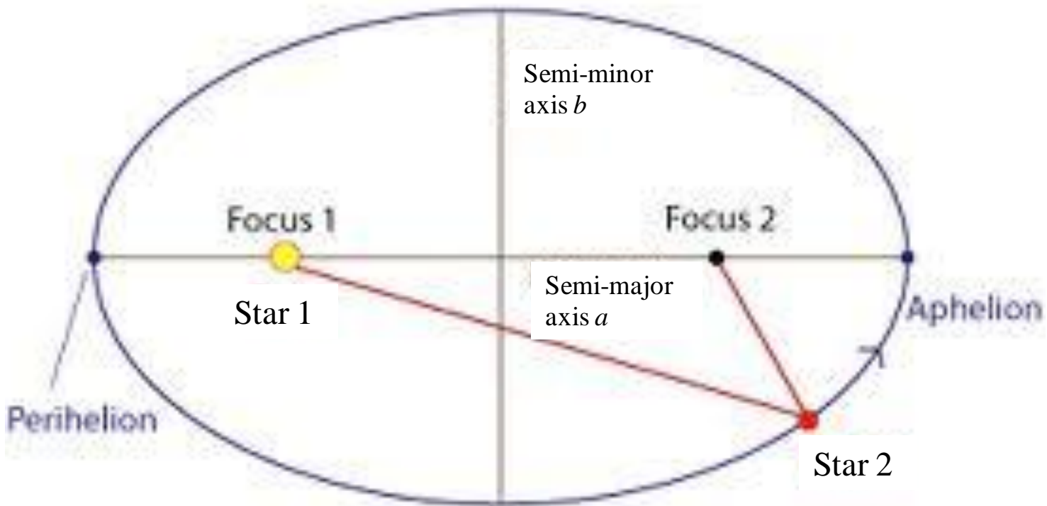
Elliptical orbit
